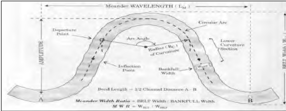
Adapted from The Reference Reach Field Book, D. Rosgen.
