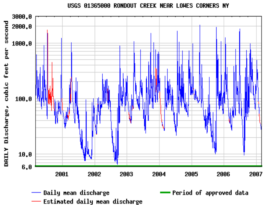
Figure 3 Hydrograph for the period of WY01 through 07, USGS gage
