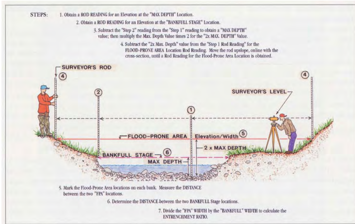
Figure 7 D. Rosgen's measure of entrenchment from Rosgen 1996
