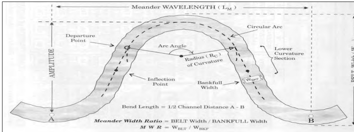
Figure 4 Adapted from The Reference Reach Field Book , D. Rosgen, 1996
